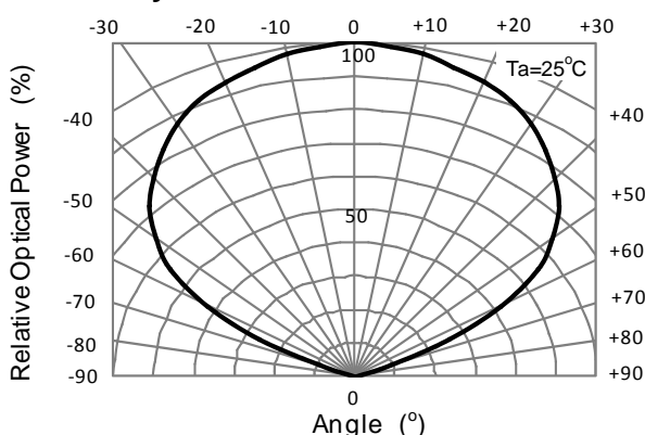
Directivity
