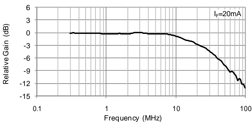
Frequency Response
