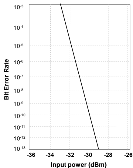
KPDX2GK Bit error rate
