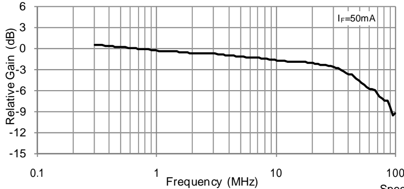
Frequency Response
