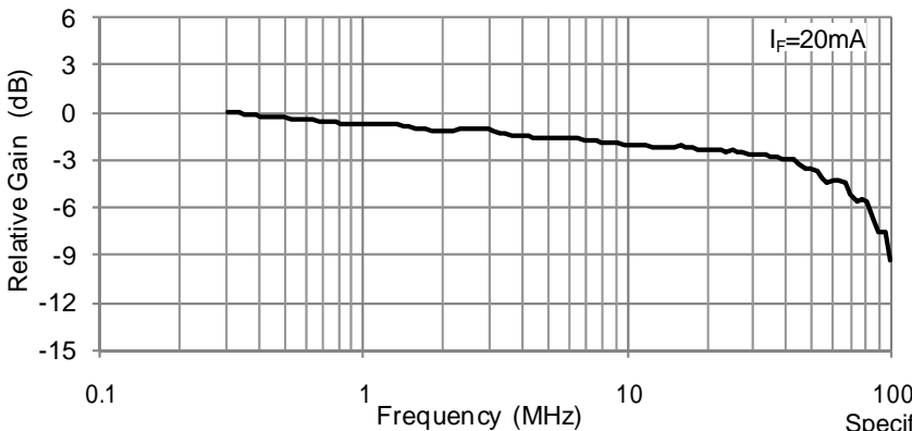
Frequency Response
