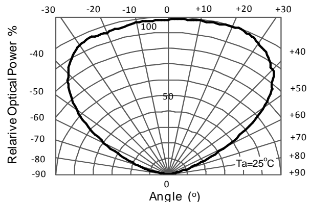
Directivity
