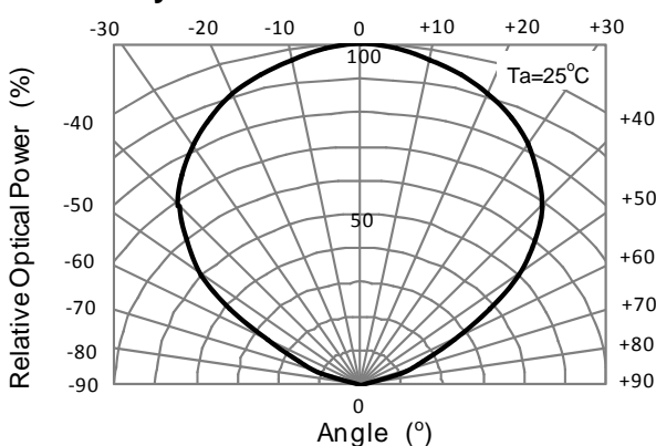
Directivity
