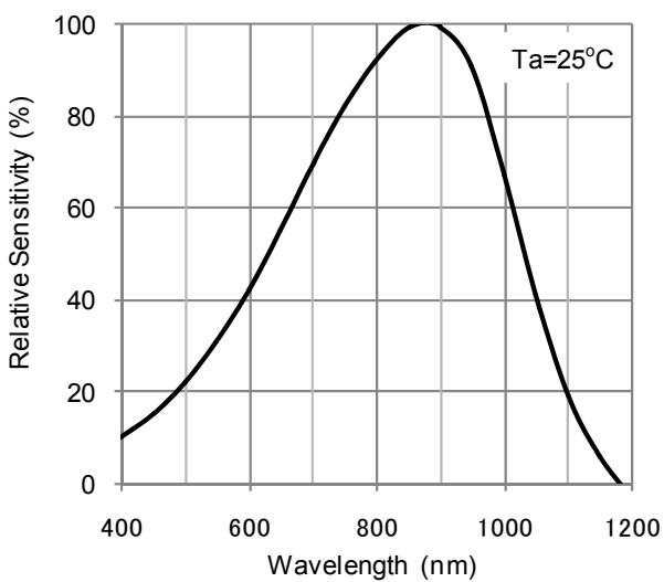
Spectral Responsivity
