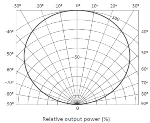
Directivity
