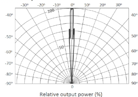
Directivity
