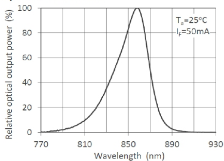
Spectral Distribution
