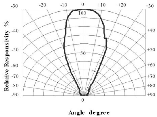
Directivity (Ta=25°C)
